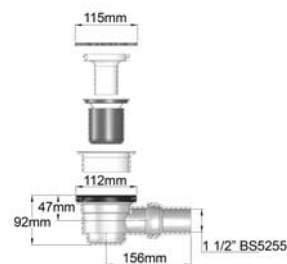
Lumin8 Tray Waste Dimensions
